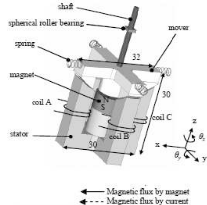
Fig. 7. Basic structure of the proposed model of the spherical resonant actuator (through the courtesy of the authors from the reference [11])
