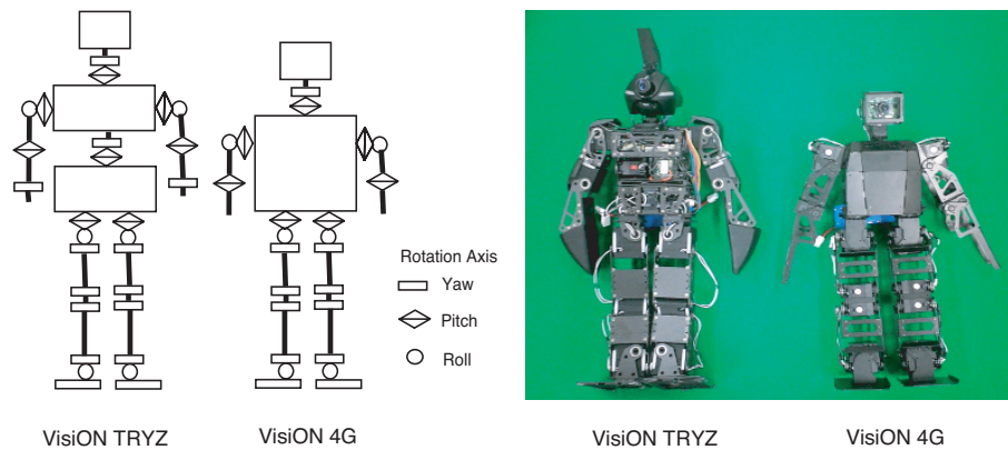
Fig. 5. The VisiON TRYZ and VisiON 4G robot: On the right side, a photo from the front view of the robots is depicted. One can see the camera (Philips chip-set) and the USB connectors for servicing in the head of the robot. On the left side is a schematic overview of the actuators and their attitude in relation to the bodies.
