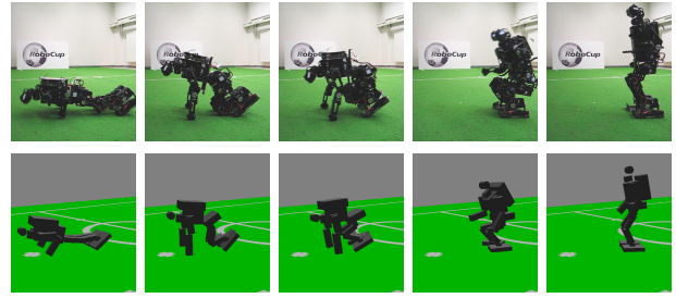
Fig. 10. Top: the real robot while getting up. Bottom: the same motion simulated with the simplified dynamics algorithm.
